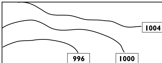
Figure 4.4(g)—Isobars
