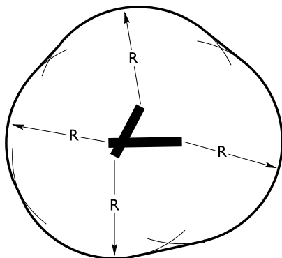
Figure 9.11—Visual Manoeuvring (Circling) Area
