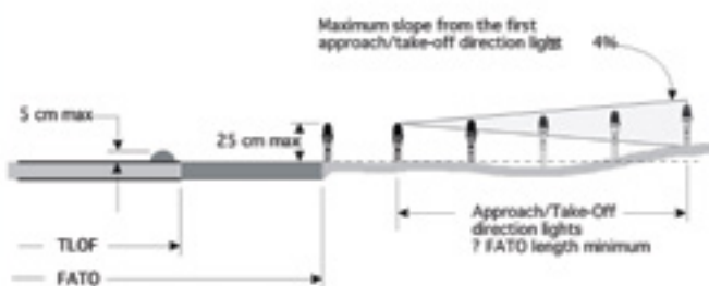
Figure 7.17—Maximum Mounting Height for TLOF, FATO, and Approach/Take-Off Direction Lights
