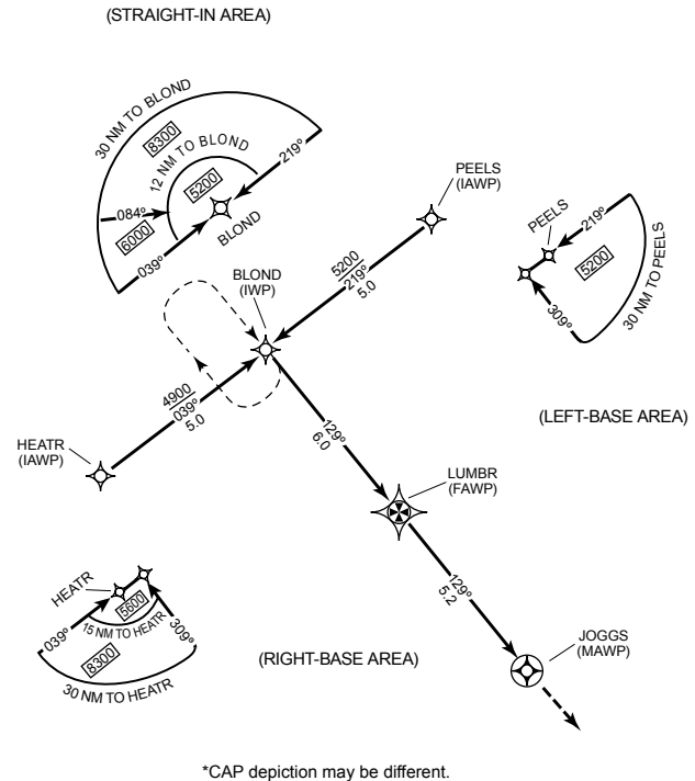
Figure 9.1—Basic “T” Approach with TAA Depiction
