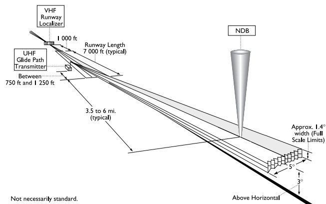
Figure 4.2—Typical ILS Installation
