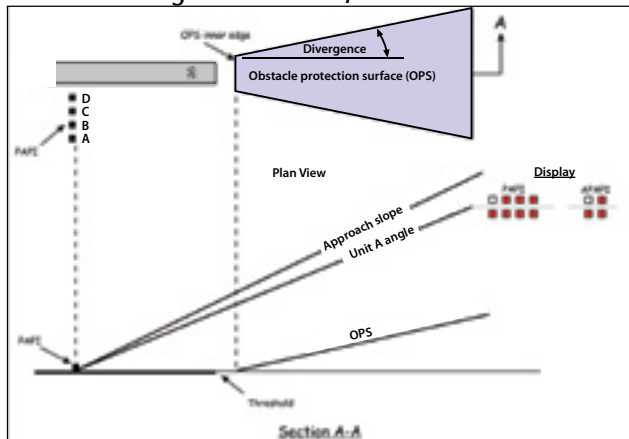
Figure 7.9—PAPI/APAPI OPS
