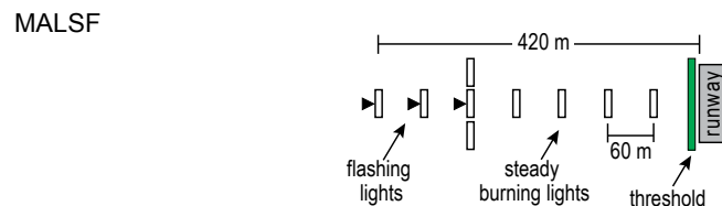
Figure 7.3—MALSF
