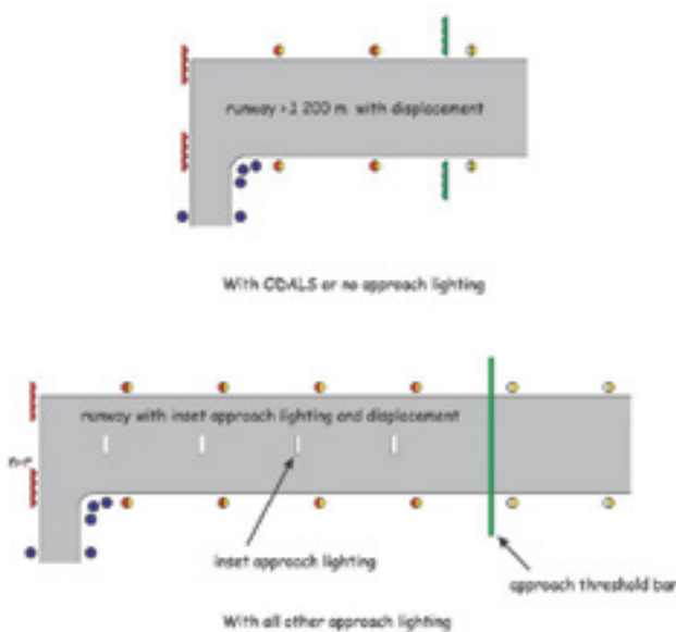
Figure 7.12—Displaced Threshold Lighting
