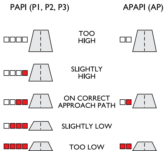
Figure 7.7—PAPI and APAPI Display
