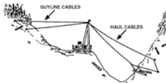
Figure 2.4—Highlead Spar
