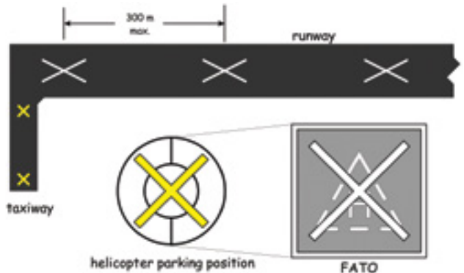
Figure 5.11—Closed Markings
