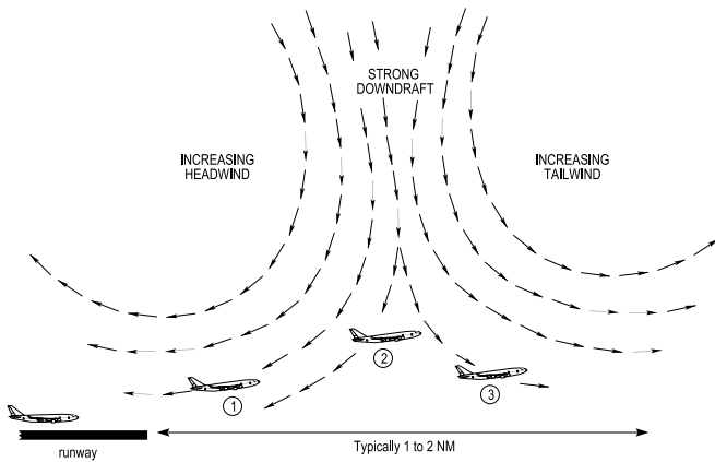
Figure 2.6—Low-Level Wind Shear
