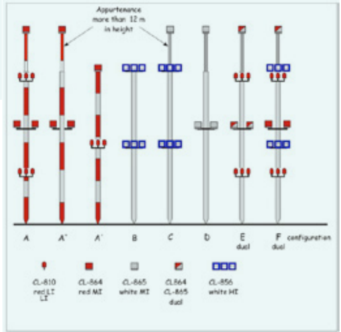
Figure 6.3—Configurations of Lighting on Skeletal Structures
