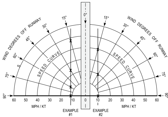
Figure 2.1—Crosswind Landing Limitations
