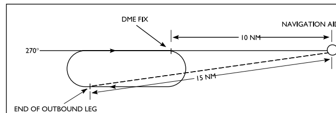
Figure 10.4—DME Hold
