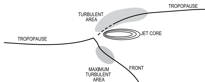
Figure 2.8—Clear Air Turbulence
