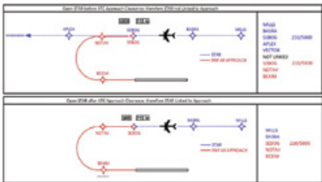
Figure 9.8 – Open STAR to RNP AR APPROACH
