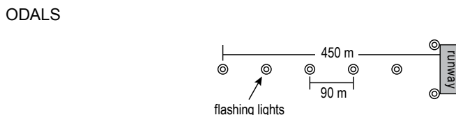
Figure 7.2—ODALS
