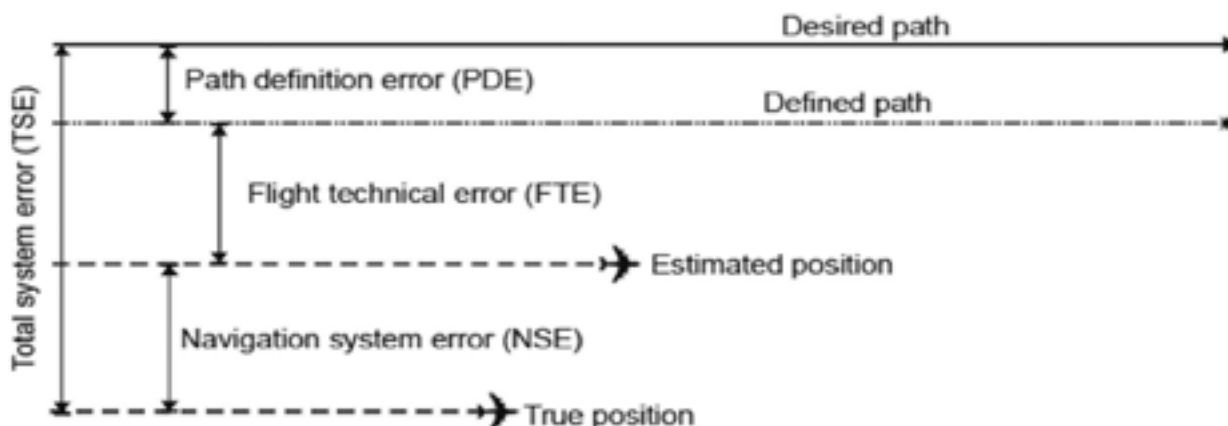
Figure 6.1—Lateral Navigation Errors
