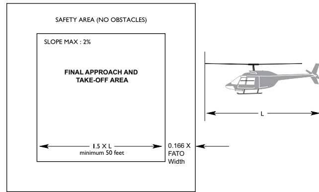
Figure 3.1—FATO/Safety Area
