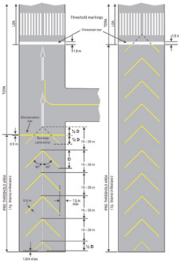
Figure 5.6—Stopway Markings
